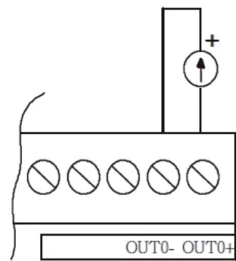
Current Output
