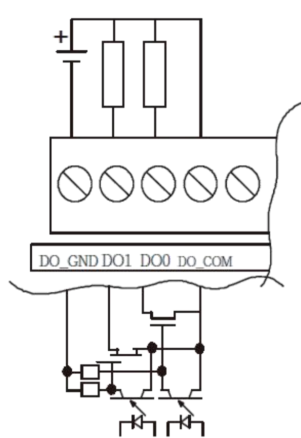
5188x-T/5189x-T Output
