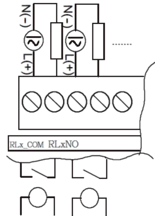
Relay Output
